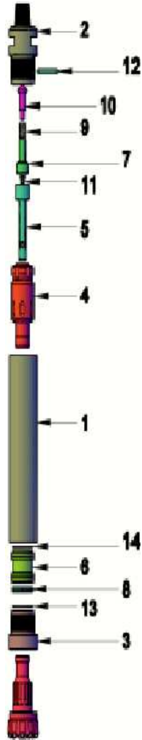
EXPLODE VIEW
